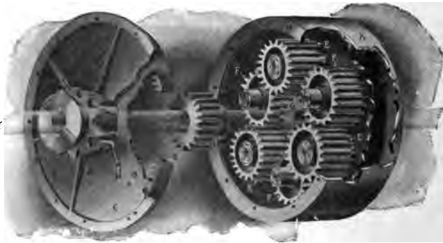
FIG. 267.—Diagram of the Cadillac Transmision, giving two forward speeds and one reverse.
